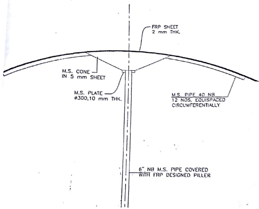
STRUCTURAL DETAIL OF FRP UMBRELLA
